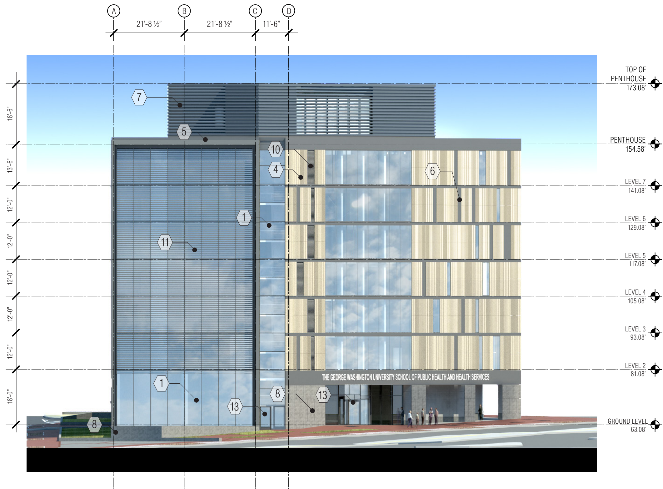
24th STREET/NEW HAMPSHIRE AVENUE INTERSECTION ELEVATION
