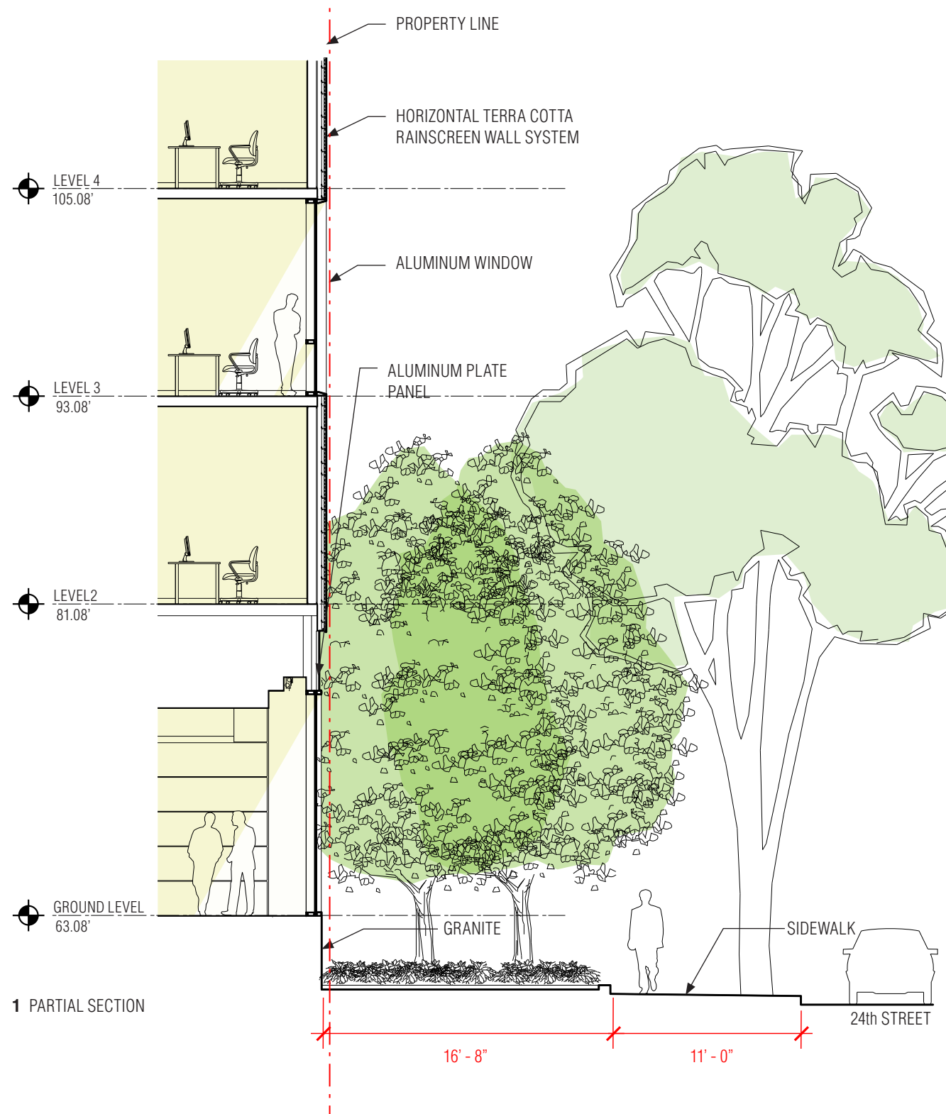
ELEVATION DETAIL AND PARTIAL SECTION AT 24th STREET FACADE
