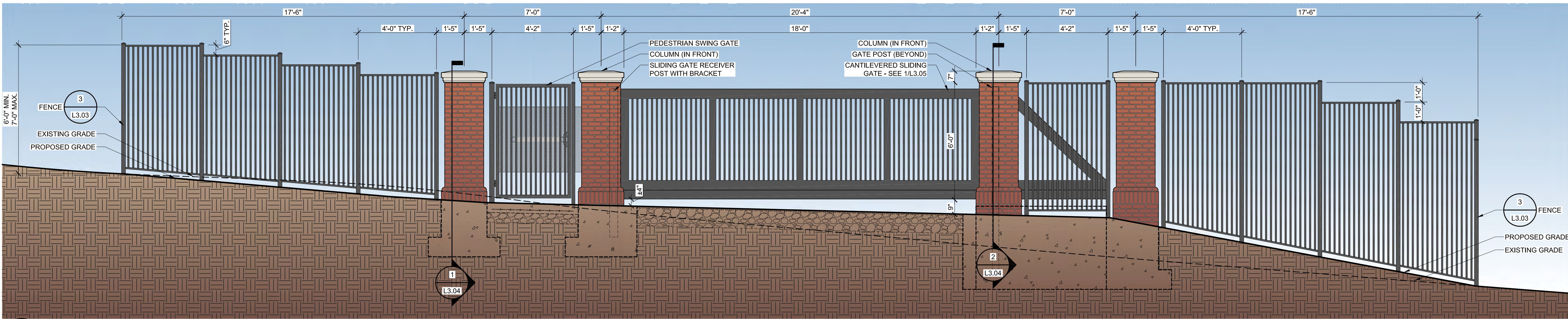
1 ENTRY ELEVATION - GATES CLOSED L3.02 Scale: 3/8" = 1'-0" ELEVATION
